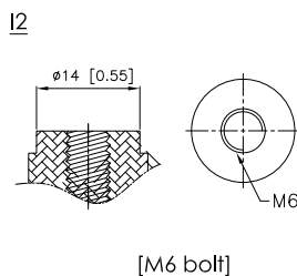
Detail A Drawing(4:1)
